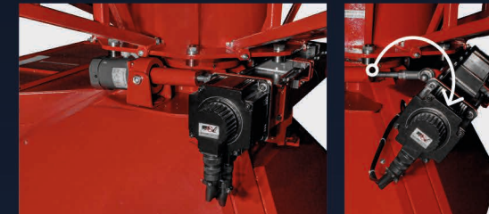
High quality servo indexer for smooth, quiet rotation at even the highest production speeds, as well as free wheel capability for manual rotation
